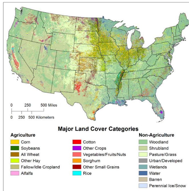
Figure 1. The USDA NASS Cropland Data Layer
