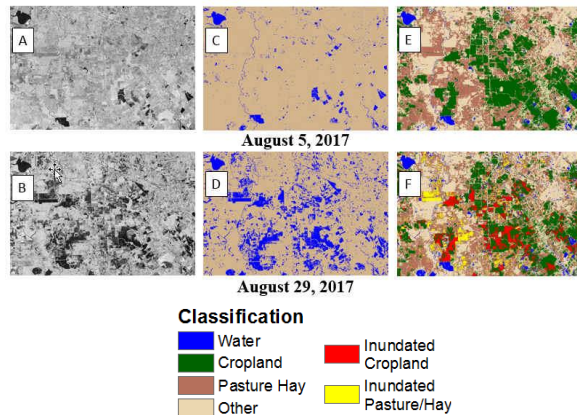
Fig. 4. (A) - Pre-flood Sentinel-1A image near Houston TX; (B) - Post flood Sentinel 1-A image, (C) - Manual thresholding result of pre-flood image classification (water – blue, other – tan); (D) - Manual thresholding result of post flood image classification; (E) - Overlay NASS 2016 Cultivated Layer and Pasture/Hay; (F) Post flood cropland classification which identifies cropland inundated based on change detection between pre- and post-flood images.
